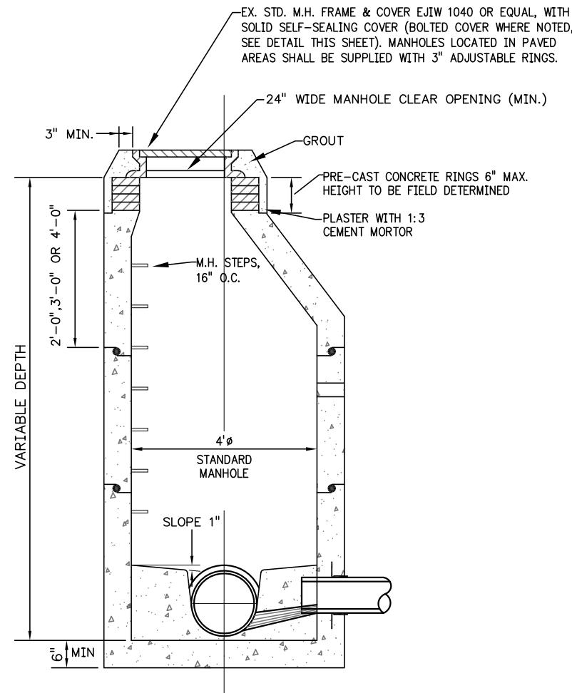
SECTION THRU STANDARD MANHOLE DETAIL - STANDARD MANHOLE NO SCALE
