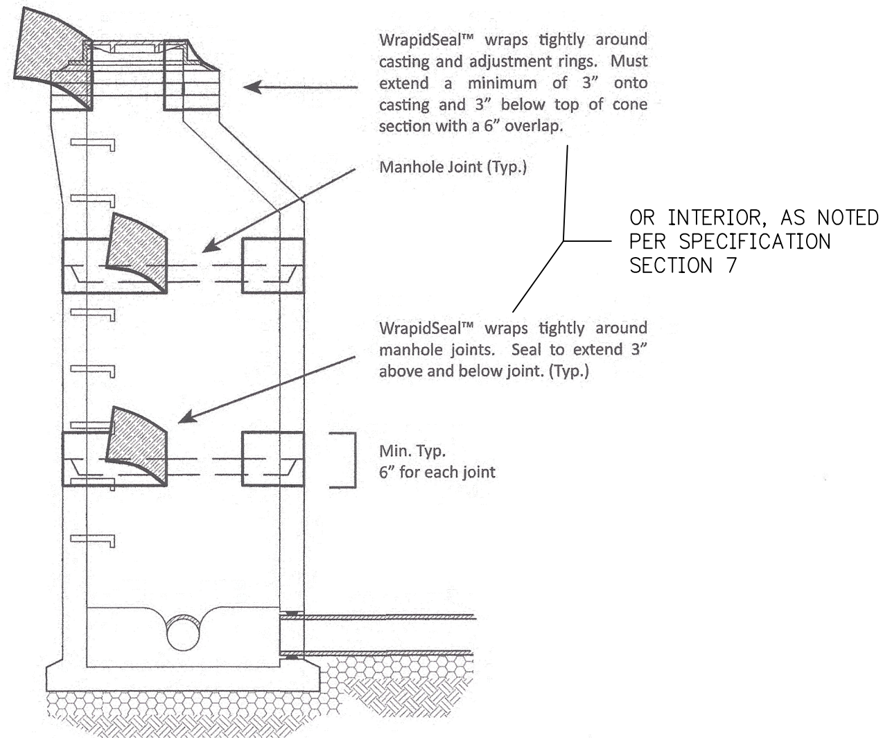
MANHOLE WATERPROOFING DETAIL NO SCALE
